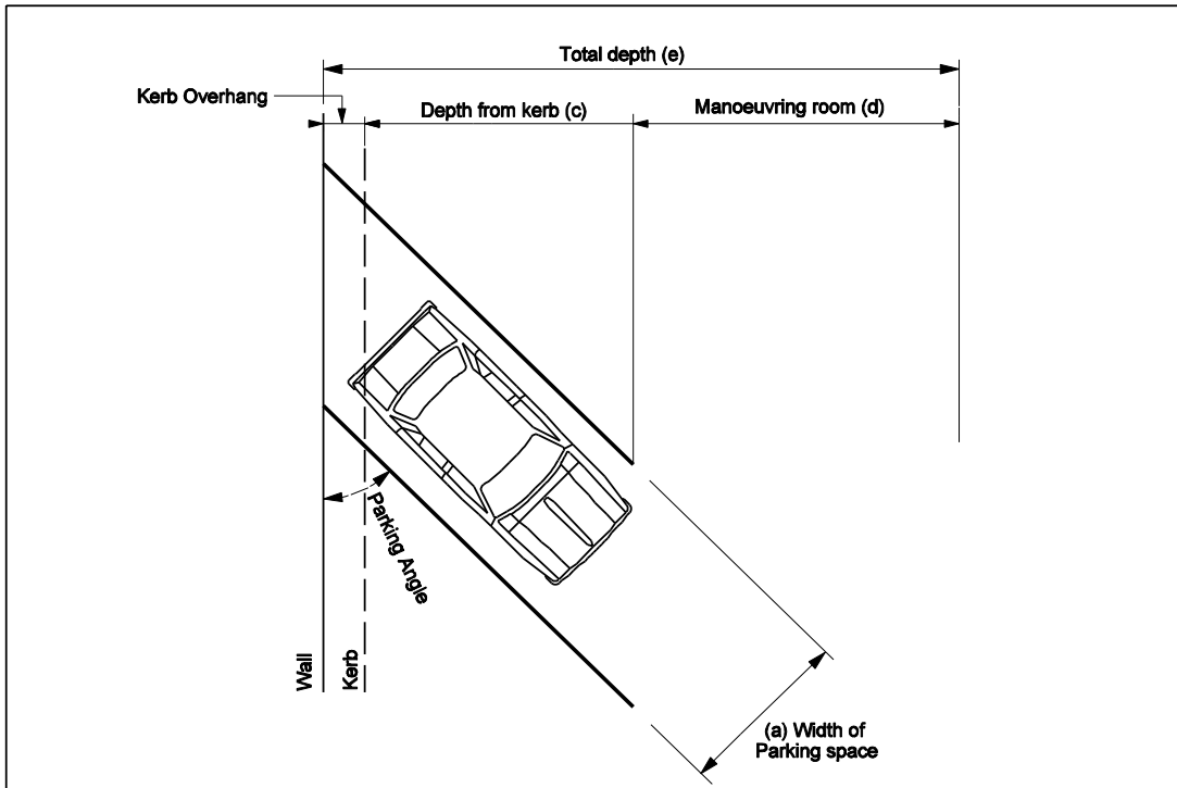
Figure 5.2-1 Car Manoeuvring and Parking Space Dimensions
