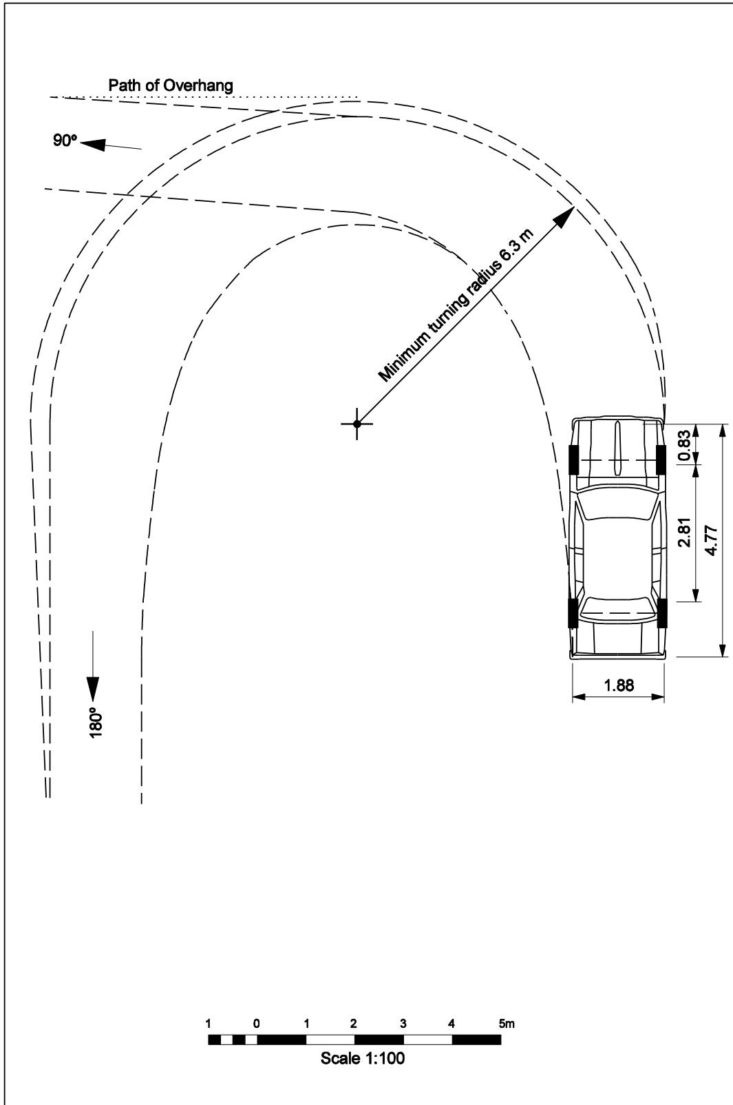
Figure 5.2-2 90 Percentile Car Tracking Curve Minimum Radius
