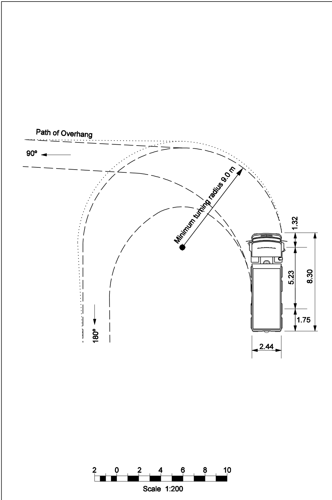
Figure 5.2-4 99 Percentile Truck Tracking Curve Minimum Radius
