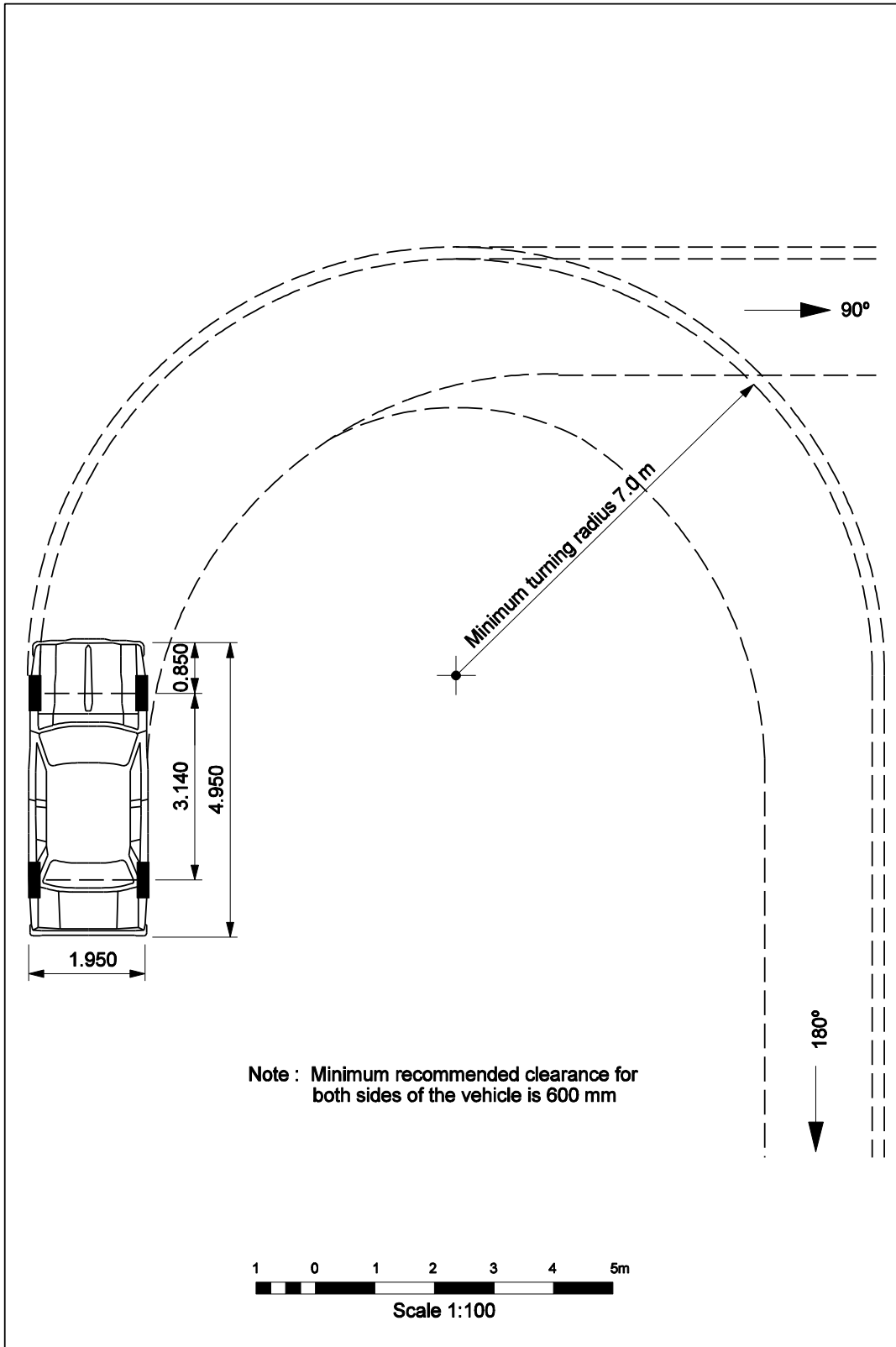
Figure 5.2-3 99 Percentile Car Tracking Curve Minimum Radius
